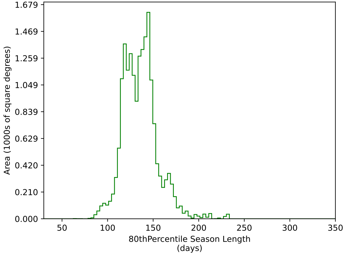
too_elab_r8_d3_ugrizy_v3.4_10yrs WFD g band: 80thPercentile Season Length
