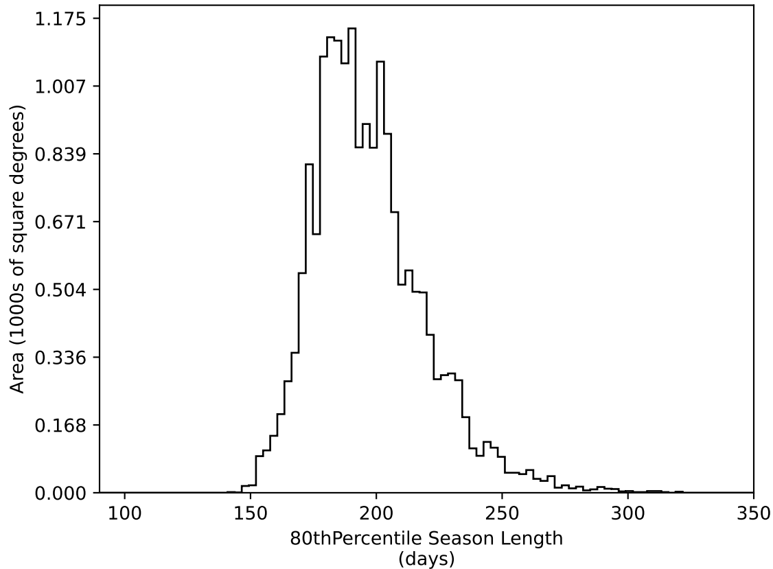
too_elab_r8_d3_ugrizy_v3.4_10yrs WFD all bands: 80thPercentile Season Length
