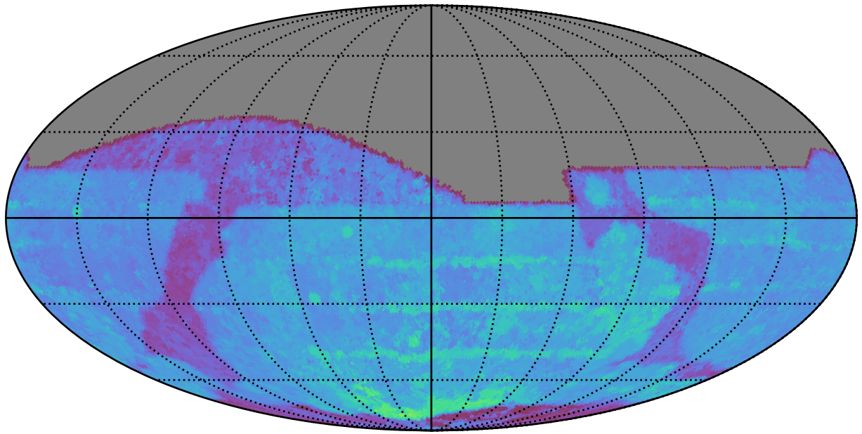
too_elab_r8_d3_ugrizy_v3.4_10yrs All sky z band: 80thPercentile Season Length
