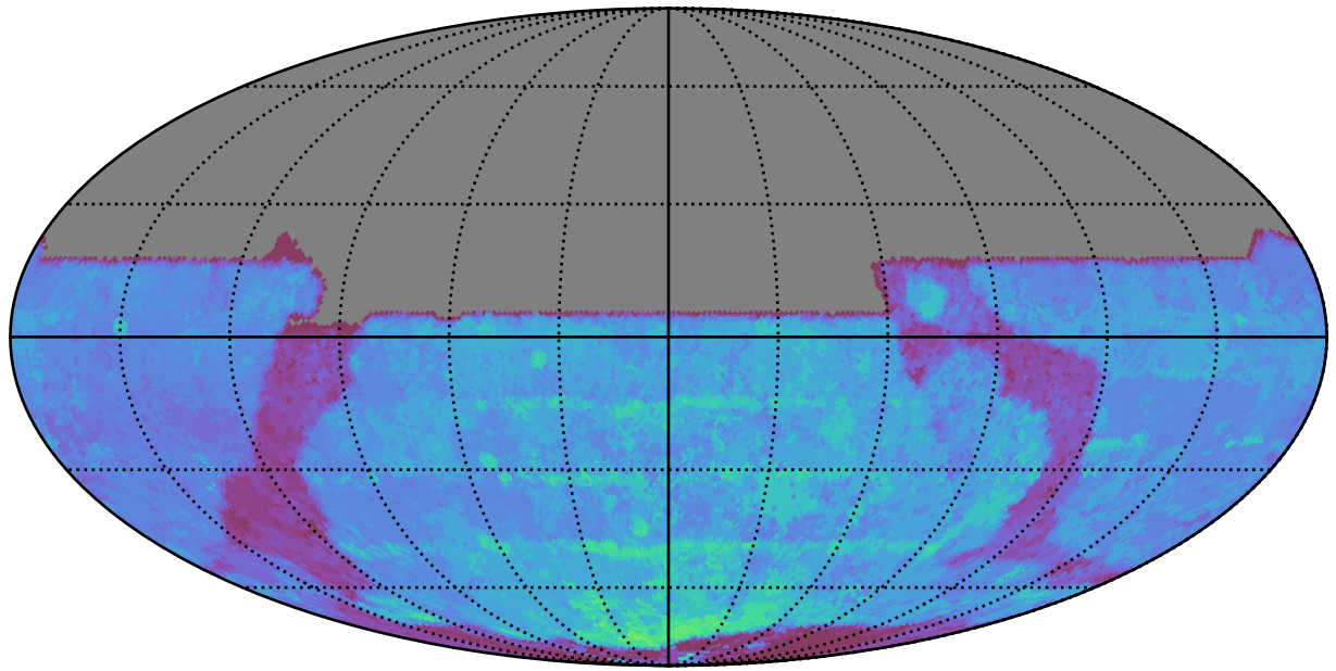
too_elab_r8_d3_ugrizy_v3.4_10yrs All sky y band: 80thPercentile Season Length
