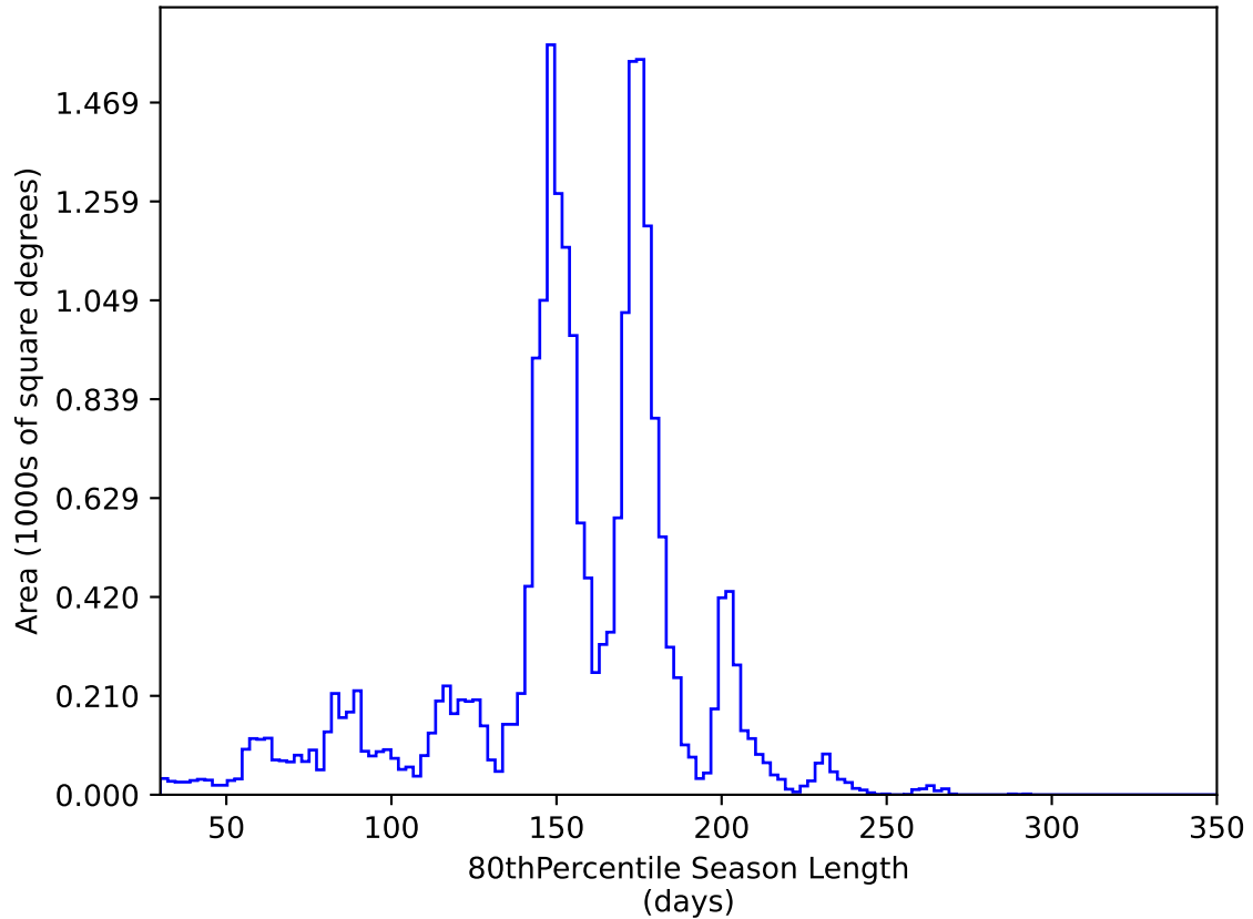
too_elab_r8_d3_ugrizy_v3.4_10yrs All sky y band: 80thPercentile Season Length
