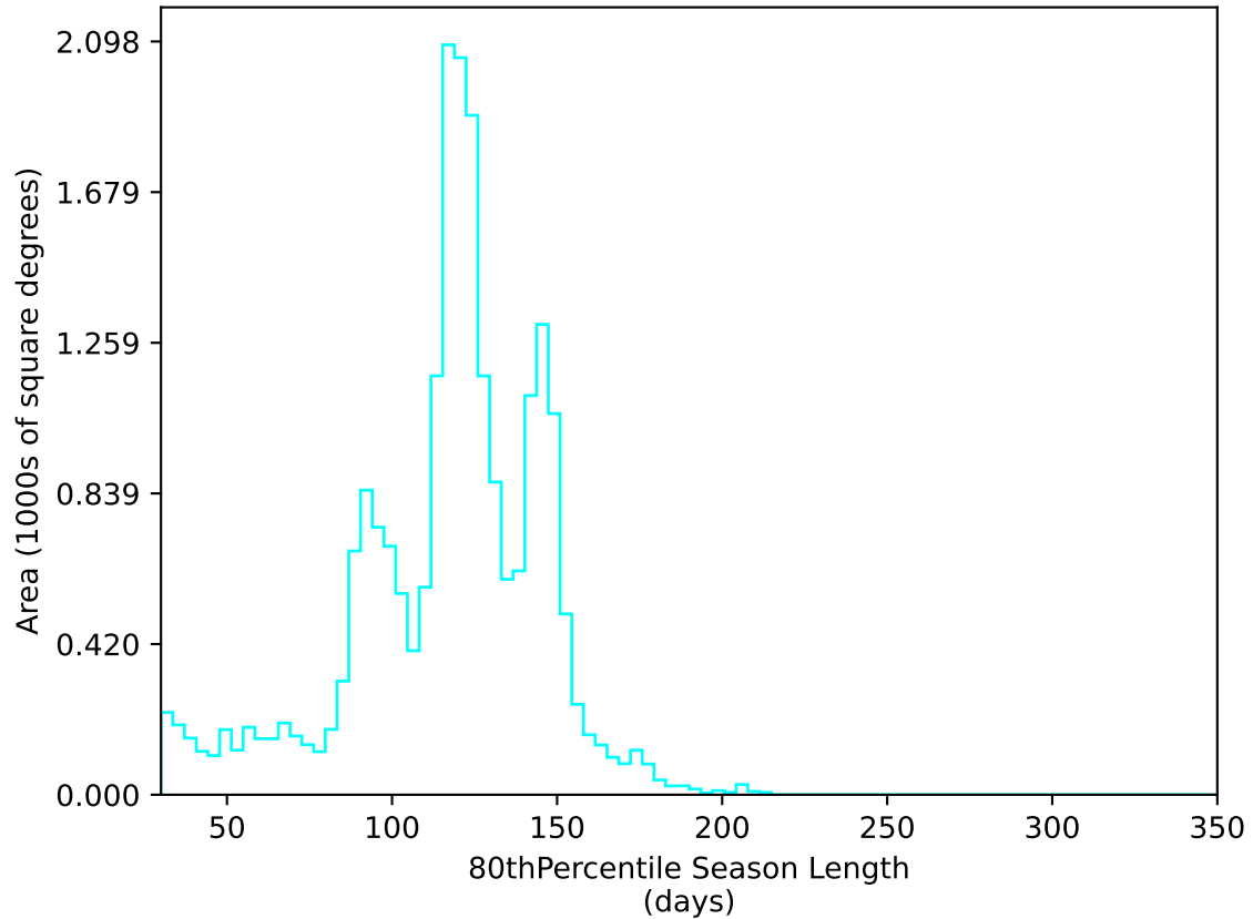
too_elab_r8_d3_ugrizy_v3.4_10yrs All sky u band: 80thPercentile Season Length
