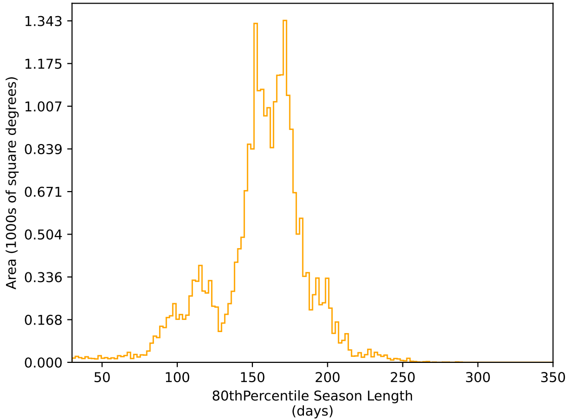
too_elab_r8_d3_ugrizy_v3.4_10yrs All sky r band: 80thPercentile Season Length
