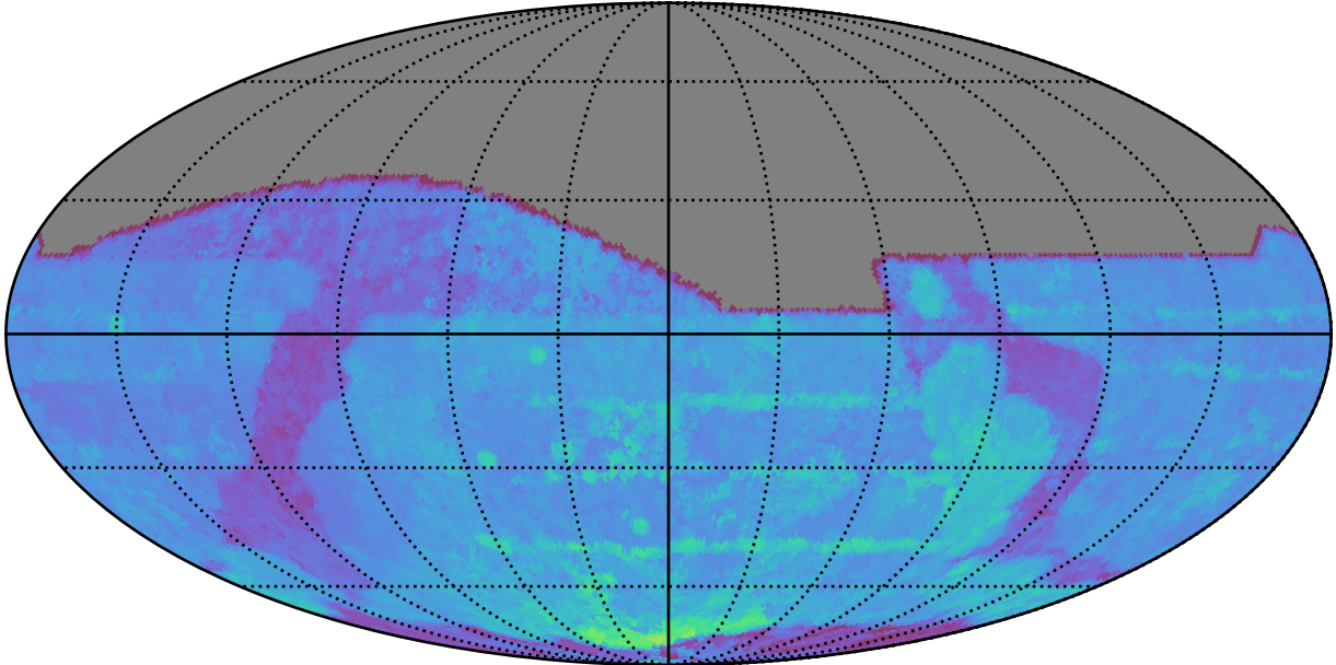
too_elab_r8_d3_ugrizy_v3.4_10yrs All sky i band: 80thPercentile Season Length
