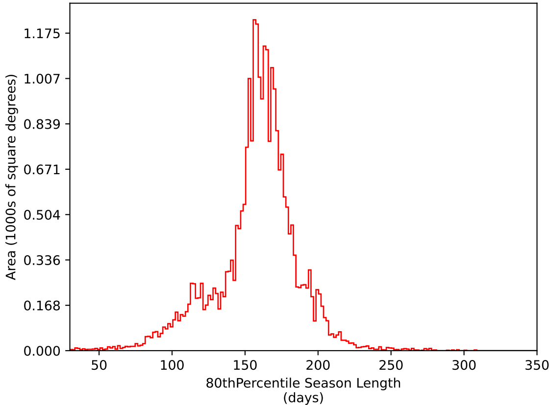
too_elab_r8_d3_ugrizy_v3.4_10yrs All sky i band: 80thPercentile Season Length
