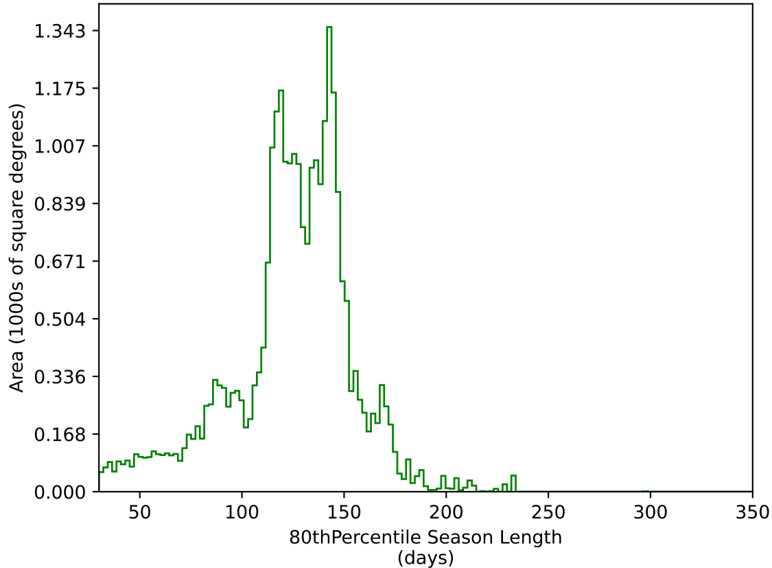
too_elab_r8_d3_ugrizy_v3.4_10yrs All sky g band: 80thPercentile Season Length
