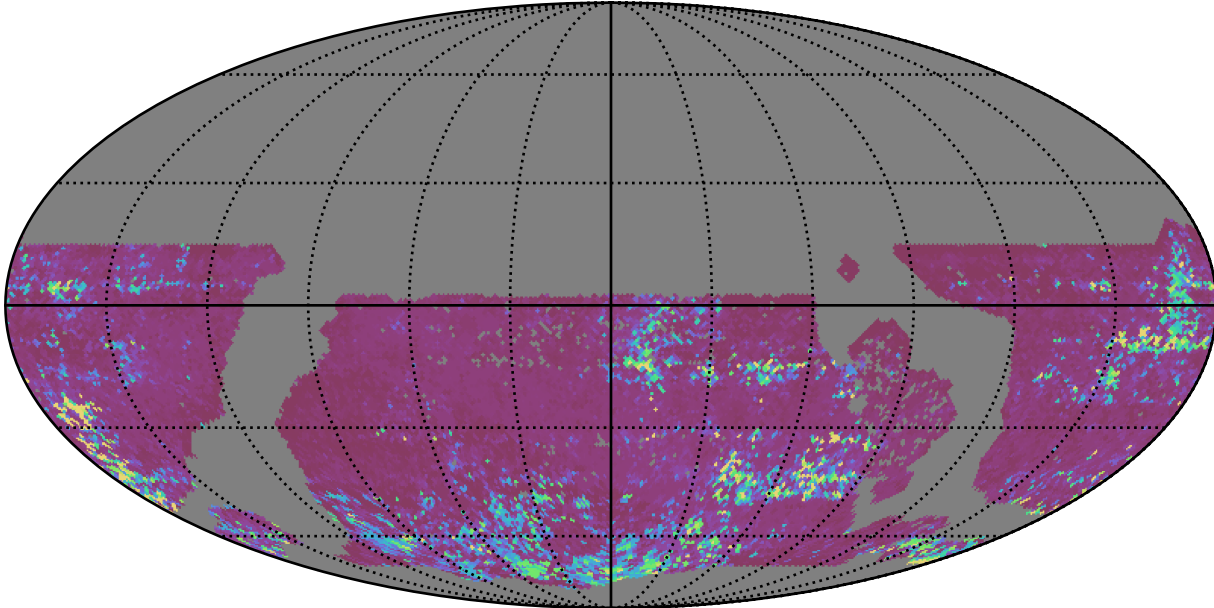
too_elab_r8_d3_ugrizy_v3.4_10yrs WFD z band: 75th Percentile Intranight Timespan
