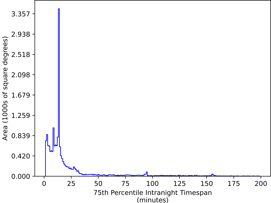
too_elab_r8_d3_ugrizy_v3.4_10yrs WFD z band: 75th Percentile Intranight Timespan
