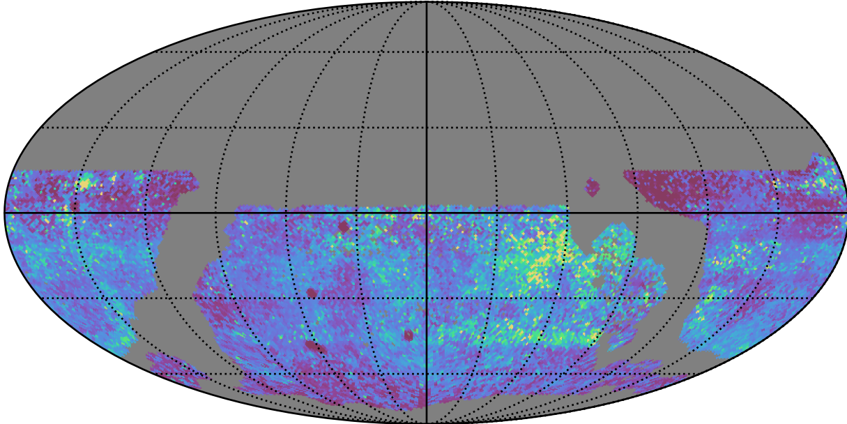
too_elab_r8_d3_ugrizy_v3.4_10yrs WFD y band: 75th Percentile Intranight Timespan
