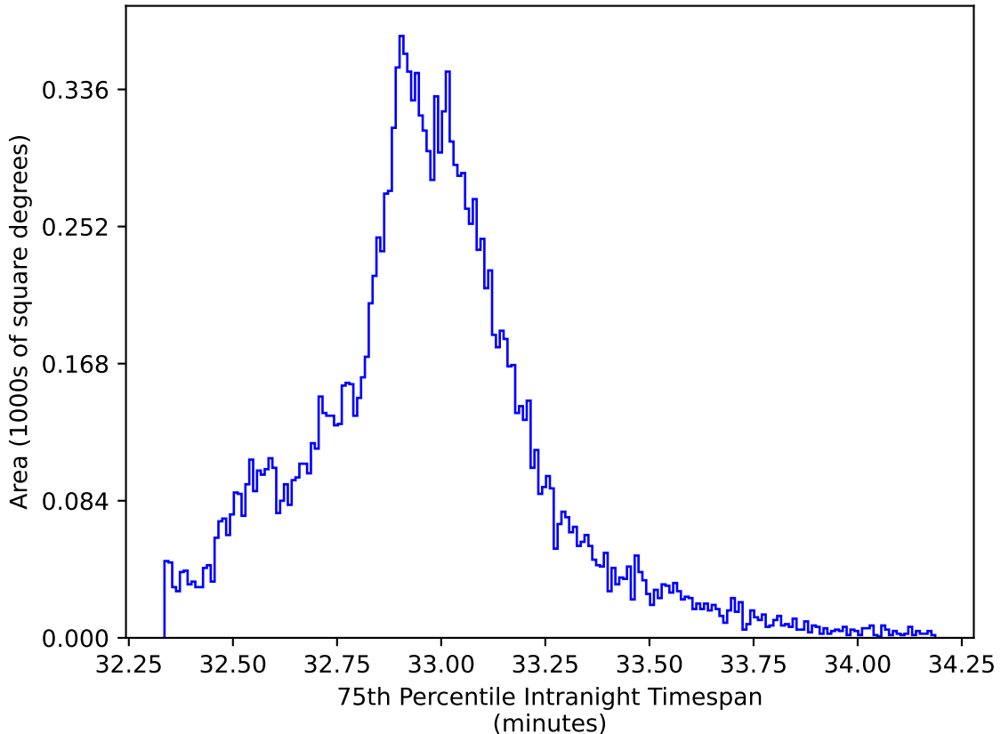
too_elab_r8_d3_ugrizy_v3.4_10yrs WFD y band: 75th Percentile Intranight Timespan
