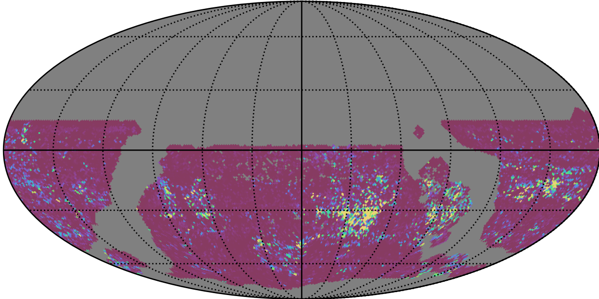
too_elab_r8_d3_ugrizy_v3.4_10yrs WFD u band: 75th Percentile Intranight Timespan
