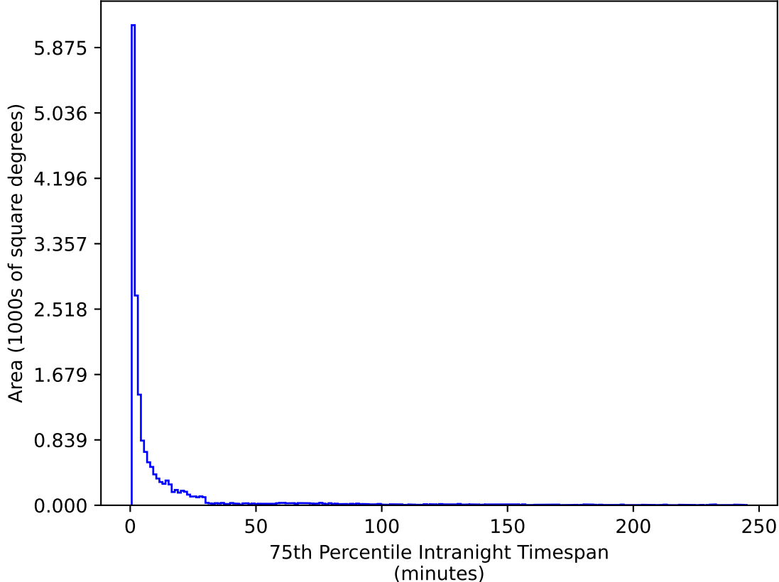
too_elab_r8_d3_ugrizy_v3.4_10yrs WFD u band: 75th Percentile Intranight Timespan
