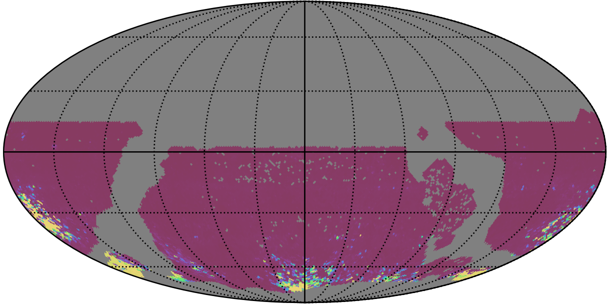
too_elab_r8_d3_ugrizy_v3.4_10yrs WFD ri bands: 75th Percentile Intranight Timespan
