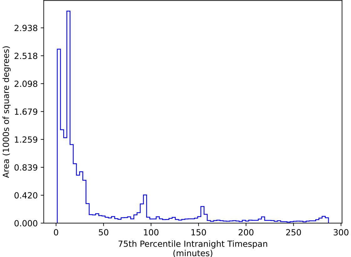
too_elab_r8_d3_ugrizy_v3.4_10yrs WFD r band: 75th Percentile Intranight Timespan
