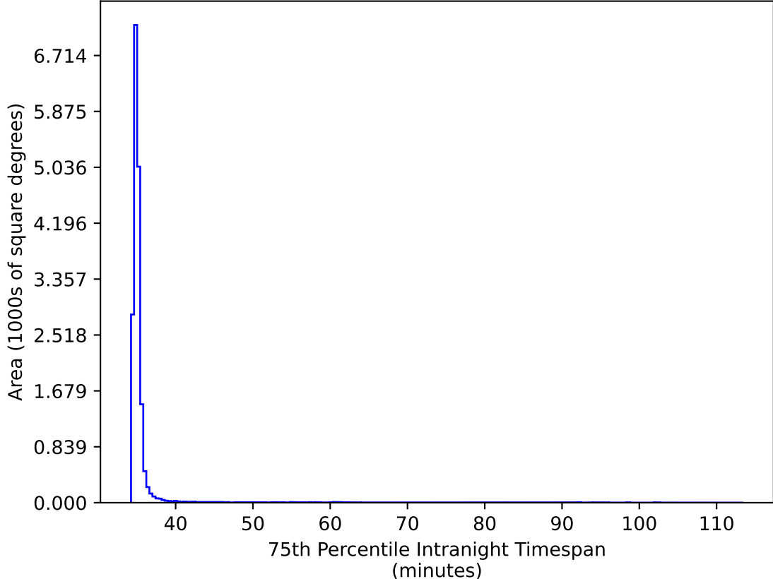
too_elab_r8_d3_ugrizy_v3.4_10yrs WFD gr bands: 75th Percentile Intranight Timespan
