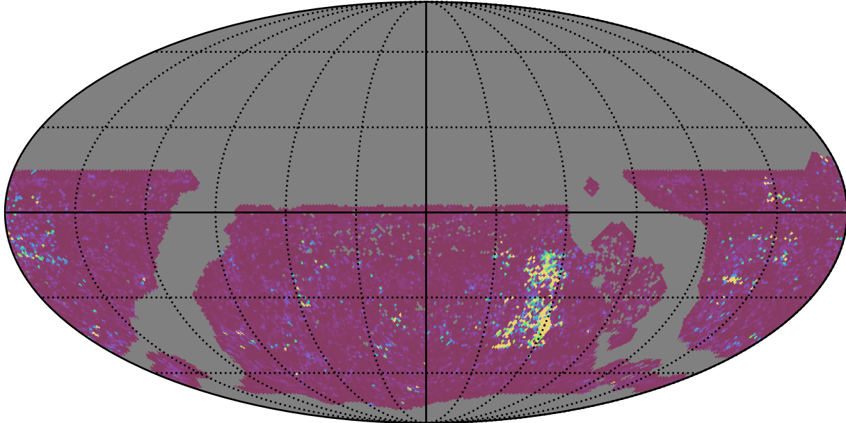
too_elab_r8_d3_ugrizy_v3.4_10yrs WFD g band: 75th Percentile Intranight Timespan
