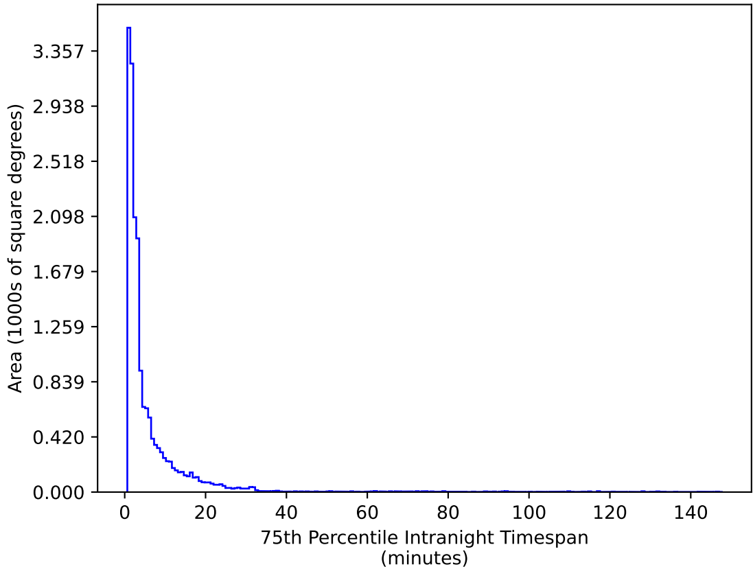
too_elab_r8_d3_ugrizy_v3.4_10yrs WFD g band: 75th Percentile Intranight Timespan
