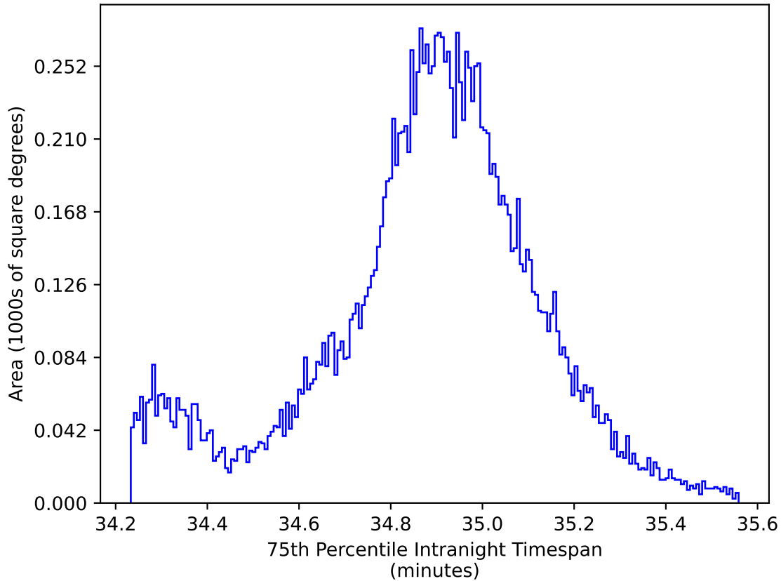
too_elab_r8_d3_ugrizy_v3.4_10yrs WFD all bands: 75th Percentile Intranight Timespan
