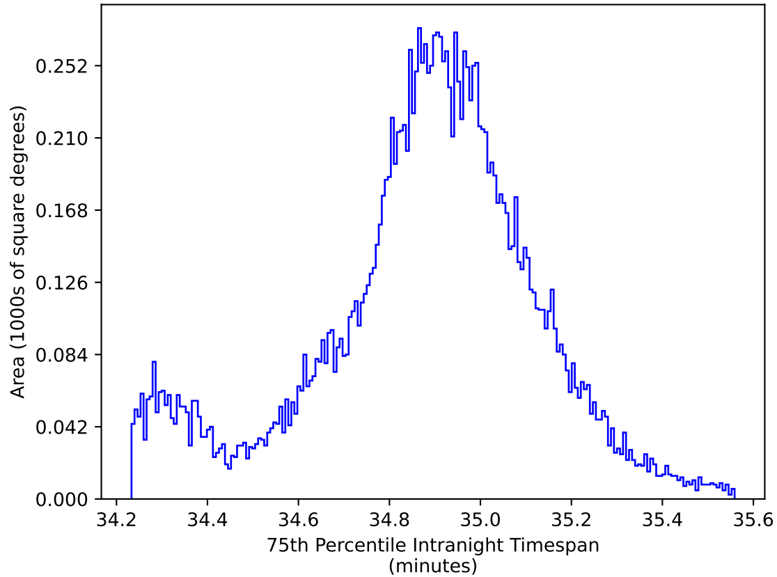
too_elab_r8_d3_ugrizy_v3.4_10yrs WFD: 75th Percentile Intranight Timespan
