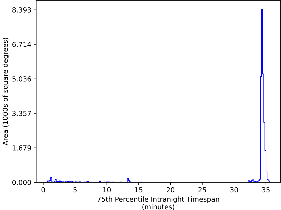
too_elab_r8_d3_ugrizy_v3.4_10yrs All sky zy bands: 75th Percentile Intranight Timespan
