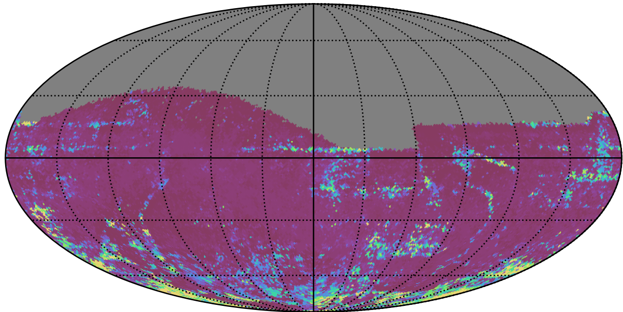
too_elab_r8_d3_ugrizy_v3.4_10yrs All sky z band: 75th Percentile Intranight Timespan
