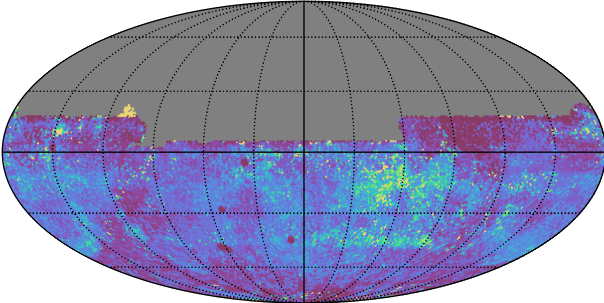
too_elab_r8_d3_ugrizy_v3.4_10yrs All sky y band: 75th Percentile Intranight Timespan
