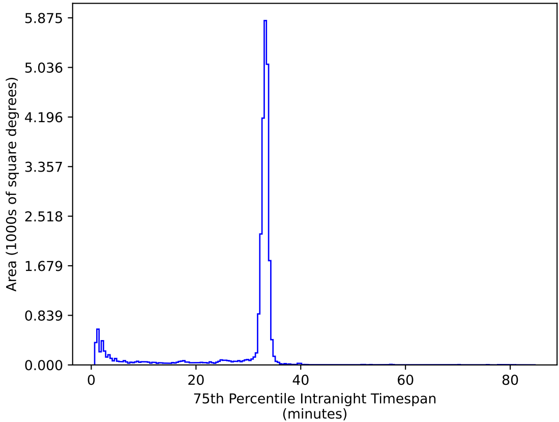
too_elab_r8_d3_ugrizy_v3.4_10yrs All sky ug bands: 75th Percentile Intranight Timespan
