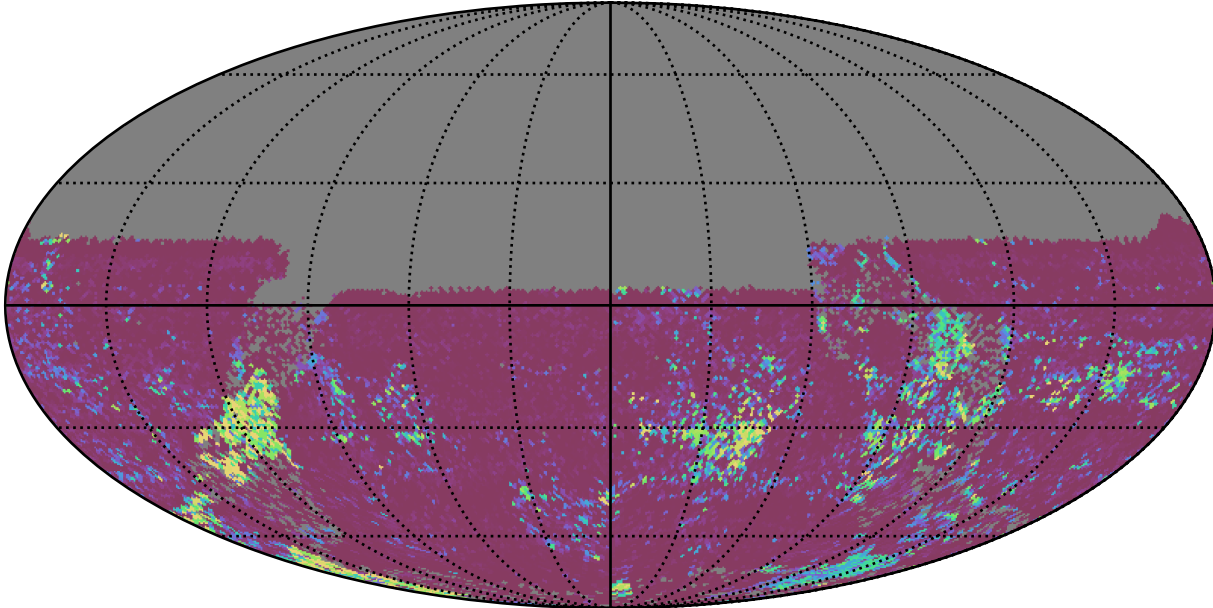
too_elab_r8_d3_ugrizy_v3.4_10yrs All sky u band: 75th Percentile Intranight Timespan
