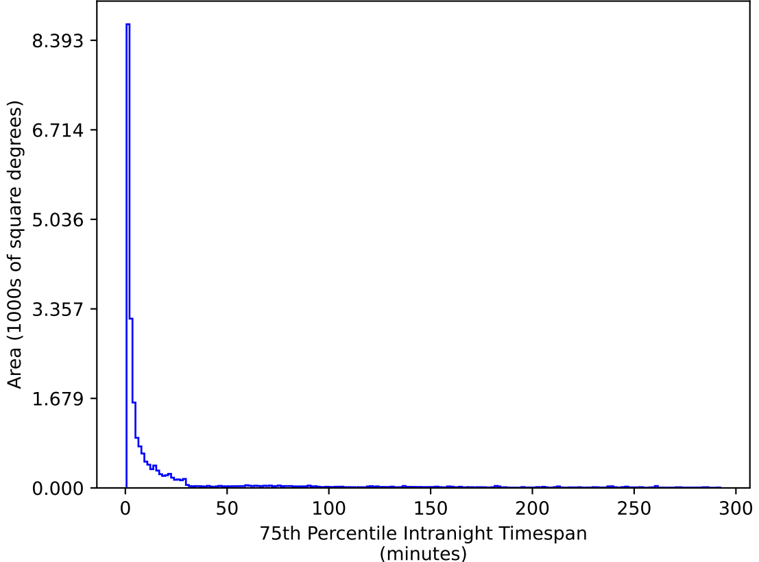
too_elab_r8_d3_ugrizy_v3.4_10yrs All sky u band: 75th Percentile Intranight Timespan
