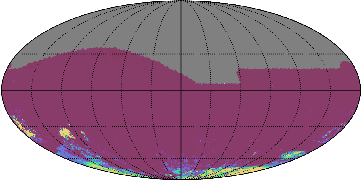
too_elab_r8_d3_ugrizy_v3.4_10yrs All sky ri bands: 75th Percentile Intranight Timespan
