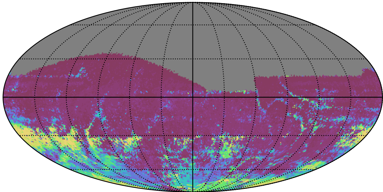
too_elab_r8_d3_ugrizy_v3.4_10yrs All sky r band: 75th Percentile Intranight Timespan
