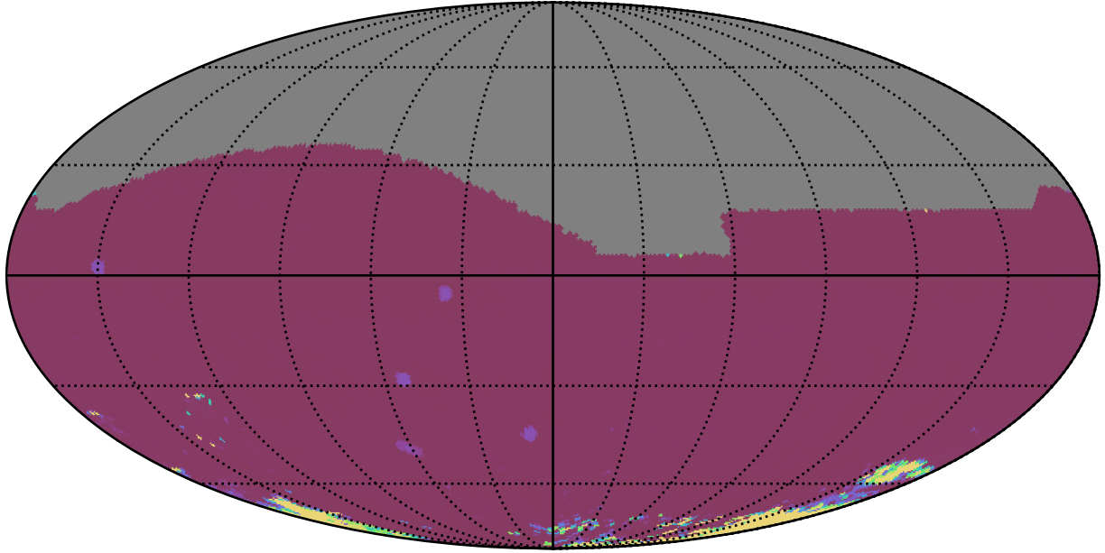
too_elab_r8_d3_ugrizy_v3.4_10yrs All sky iz bands: 75th Percentile Intranight Timespan
