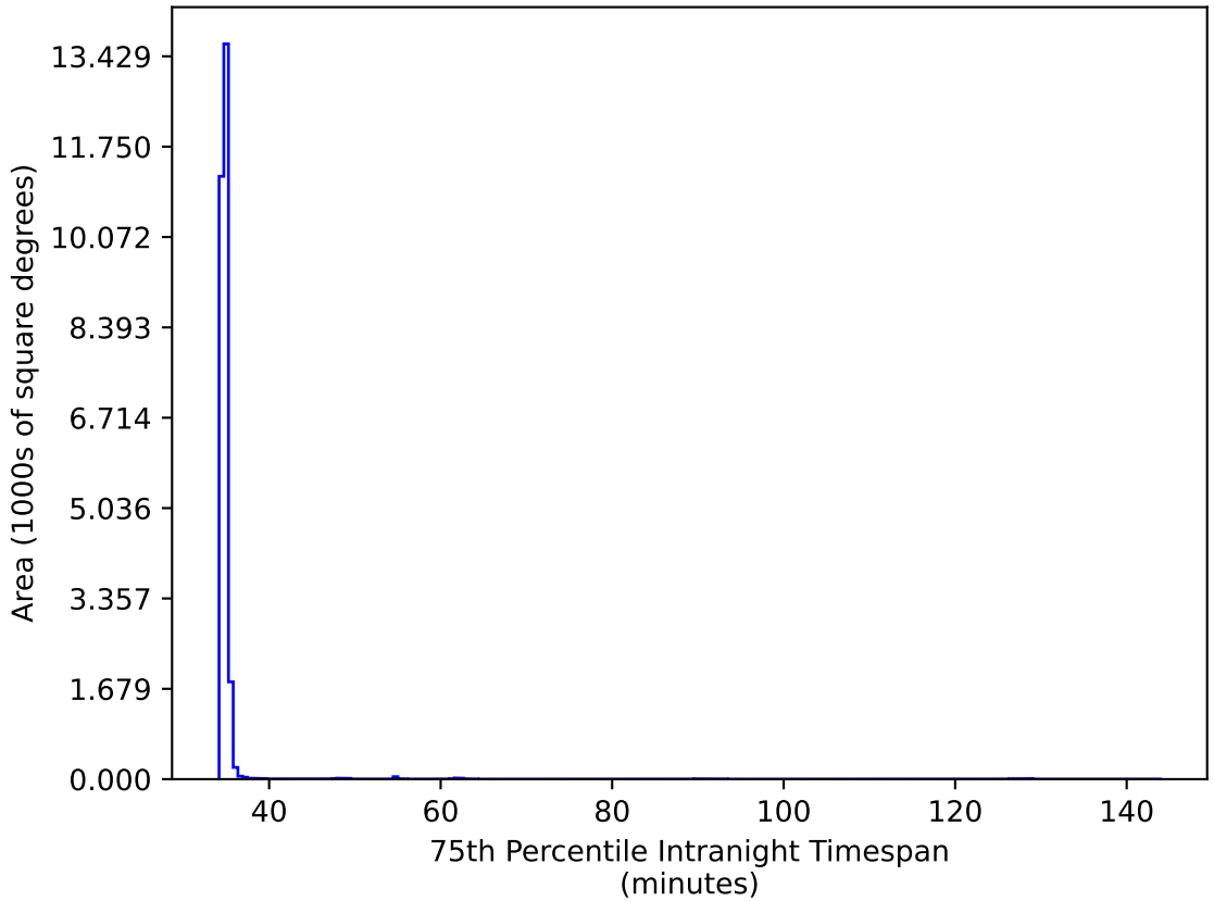
too_elab_r8_d3_ugrizy_v3.4_10yrs All sky iz bands: 75th Percentile Intranight Timespan
