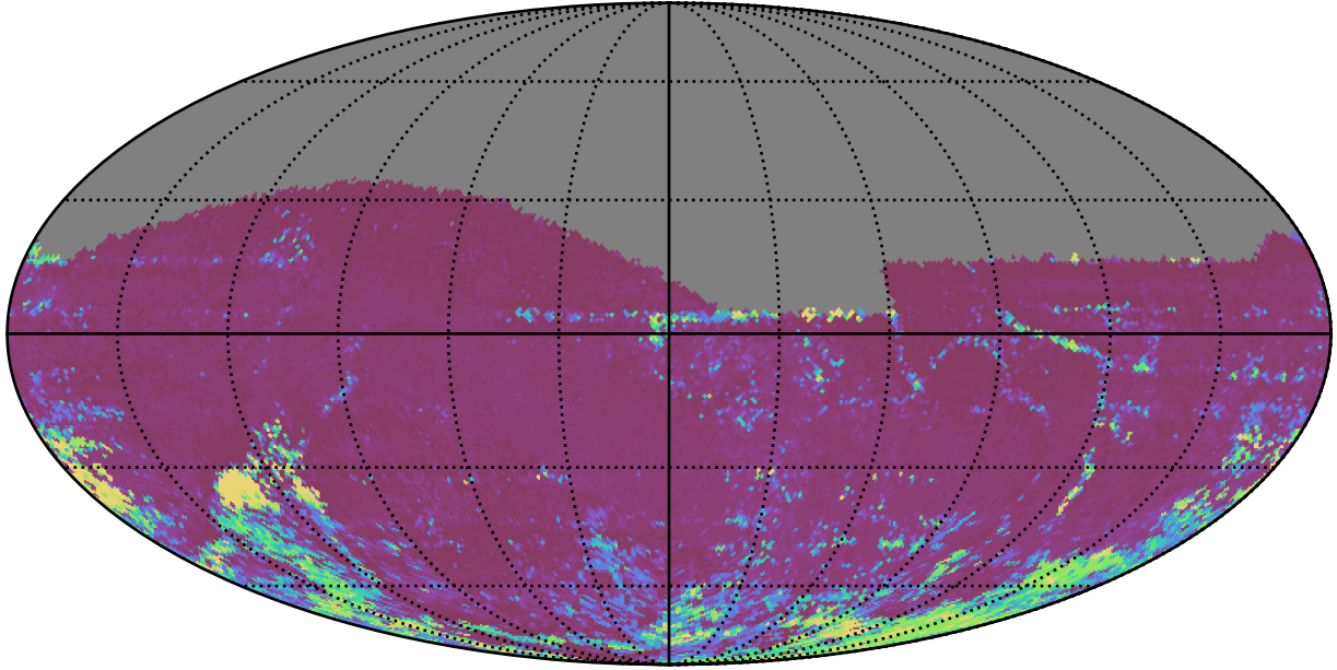
too_elab_r8_d3_ugrizy_v3.4_10yrs All sky i band: 75th Percentile Intranight Timespan
