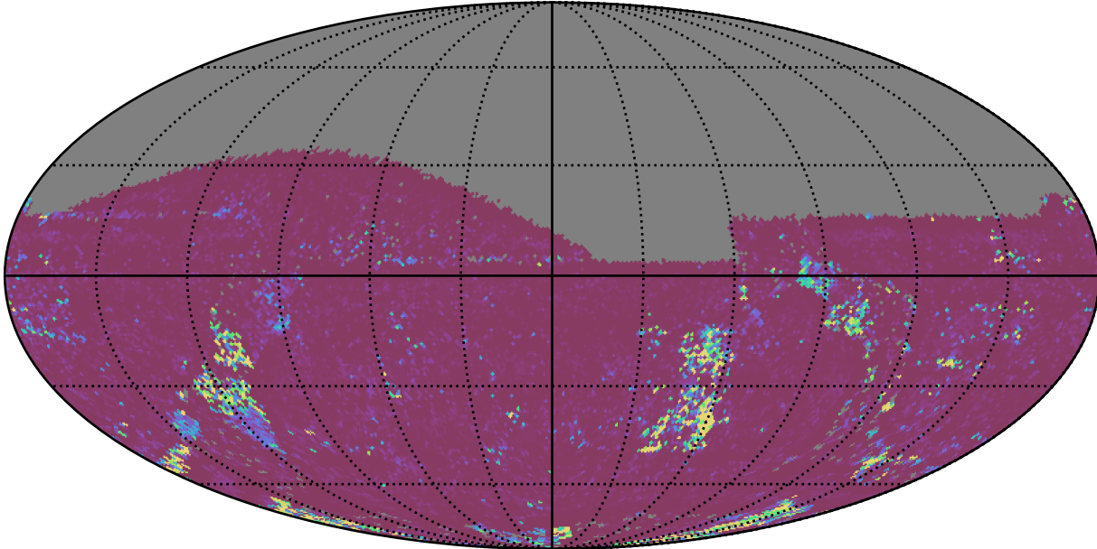
too_elab_r8_d3_ugrizy_v3.4_10yrs All sky g band: 75th Percentile Intranight Timespan
