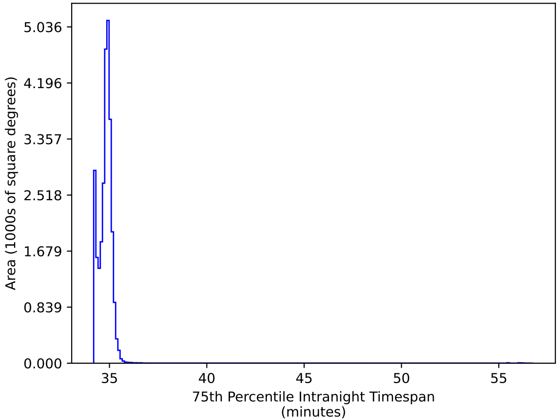
too_elab_r8_d3_ugrizy_v3.4_10yrs All sky all bands: 75th Percentile Intranight Timespan
