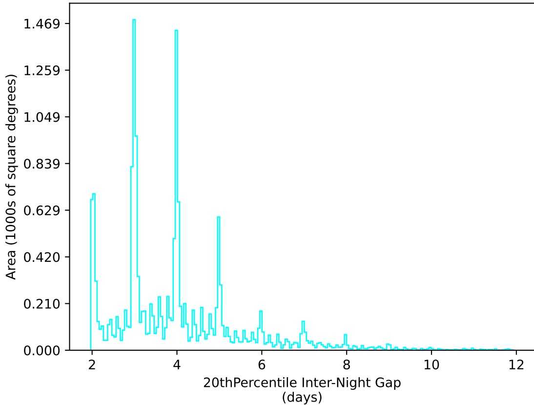
too_elab_r8_d3_ugrizy_v3.4_10yrs WFD u band: 20thPercentile Inter-Night Gap
