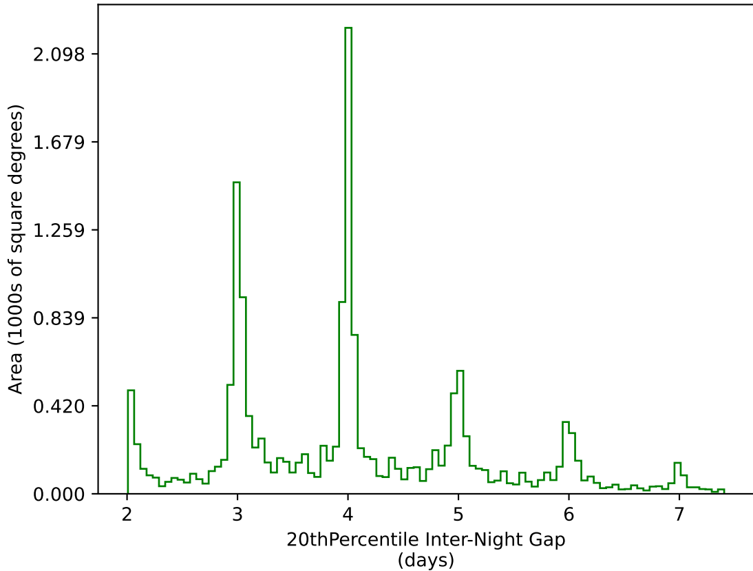
too_elab_r8_d3_ugrizy_v3.4_10yrs WFD g band: 20thPercentile Inter-Night Gap
