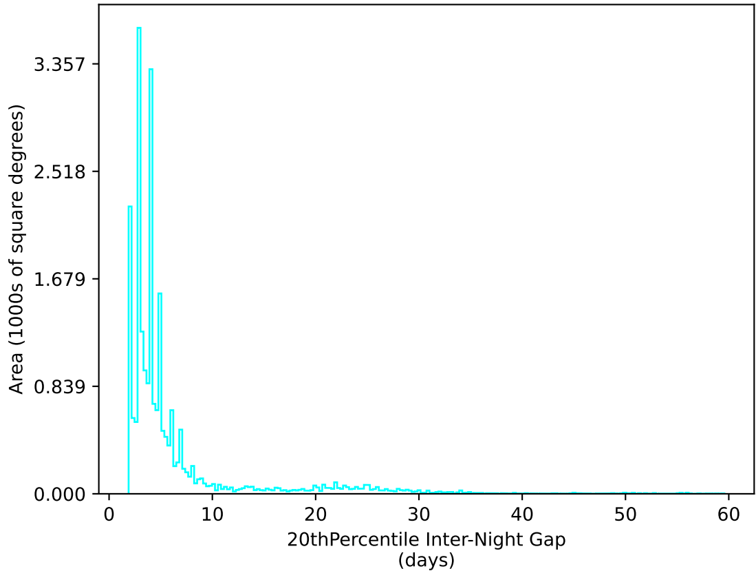
too_elab_r8_d3_ugrizy_v3.4_10yrs All sky u band: 20thPercentile Inter-Night Gap
