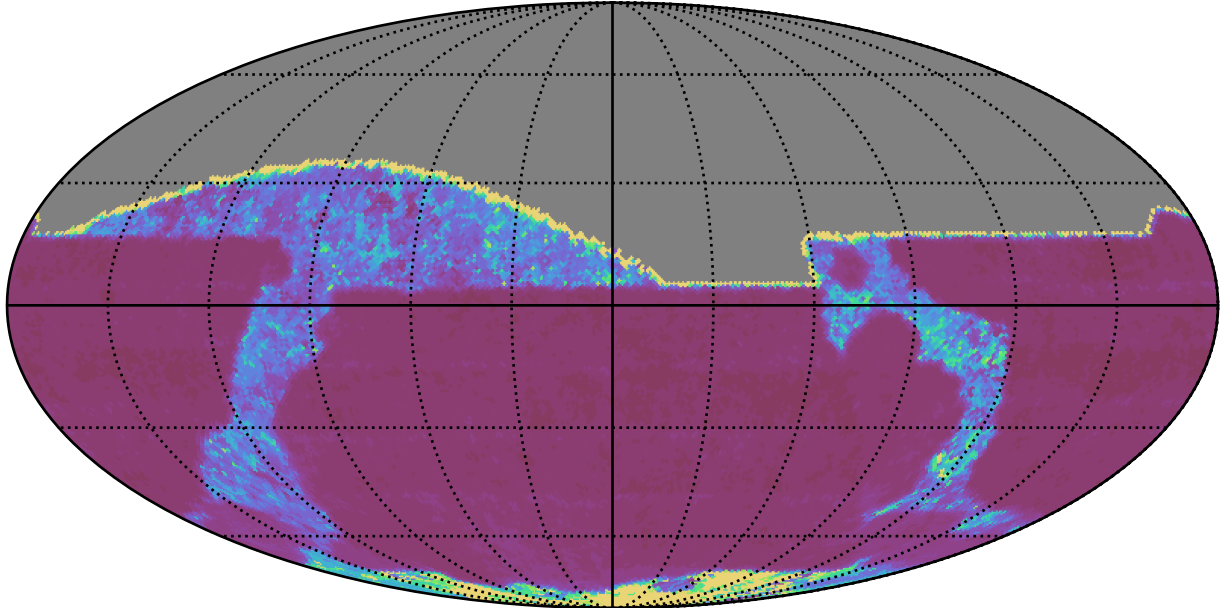
too_elab_r8_d3_ugrizy_v3.4_10yrs All sky r band: 20thPercentile Inter-Night Gap
