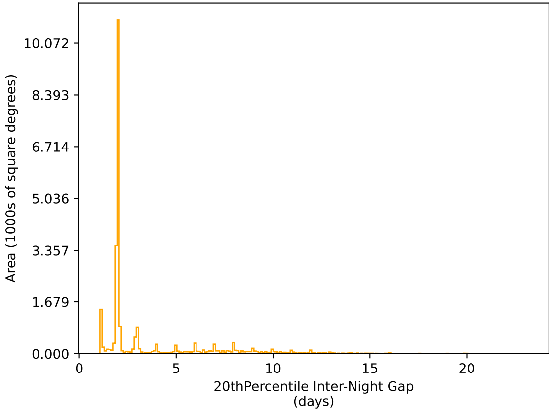
too_elab_r8_d3_ugrizy_v3.4_10yrs All sky r band: 20thPercentile Inter-Night Gap
