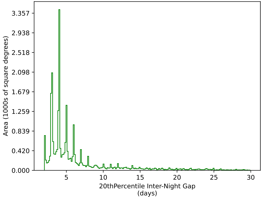
too_elab_r8_d3_ugrizy_v3.4_10yrs All sky g band: 20thPercentile Inter-Night Gap
