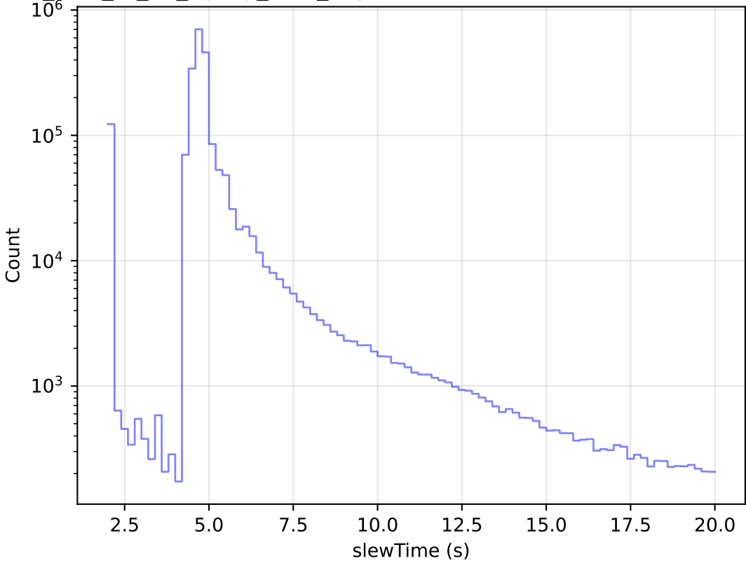
too_elab_r8_d3_ugrizy_v3.4_10yrs All visits: Zoom Slew Time Histogram
