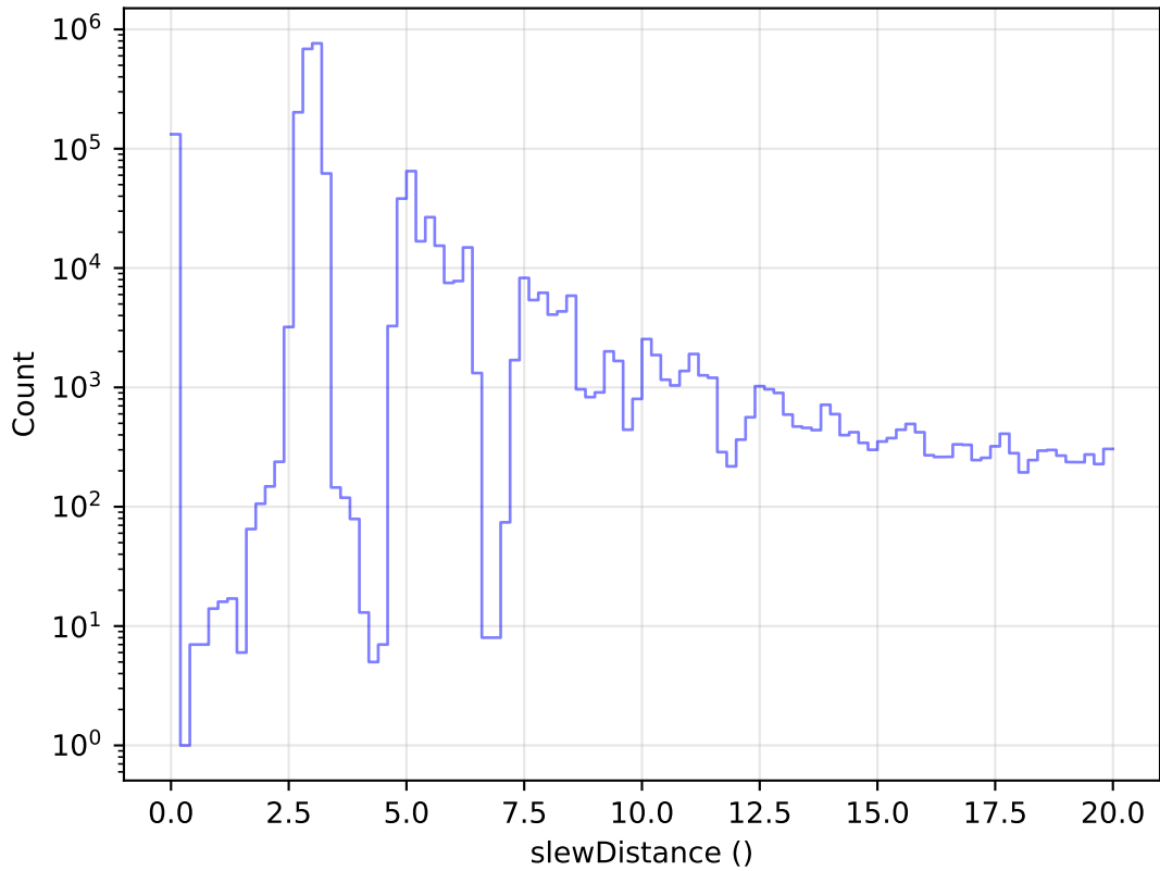
too_elab_r8_d3_ugrizy_v3.4_10yrs All visits: Zoom Slew Distance Histogram
