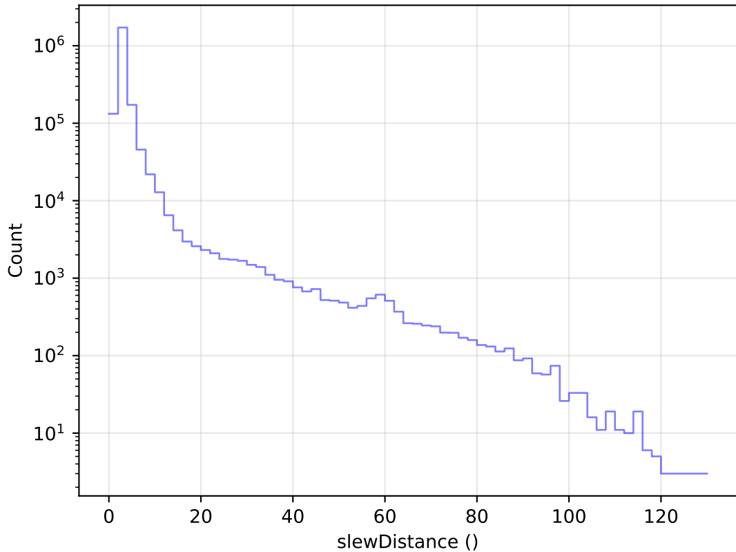
too_elab_r8_d3_ugrizy_v3.4_10yrs All visits: Slew Distance Histogram
