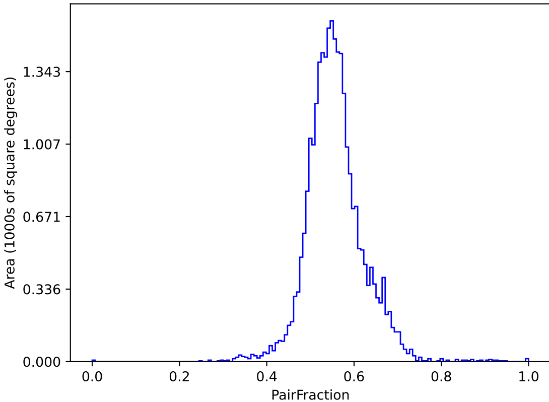
too_elab_r8_d3_ugrizy_v3.4_10yrs (g or r or i): PairFraction
