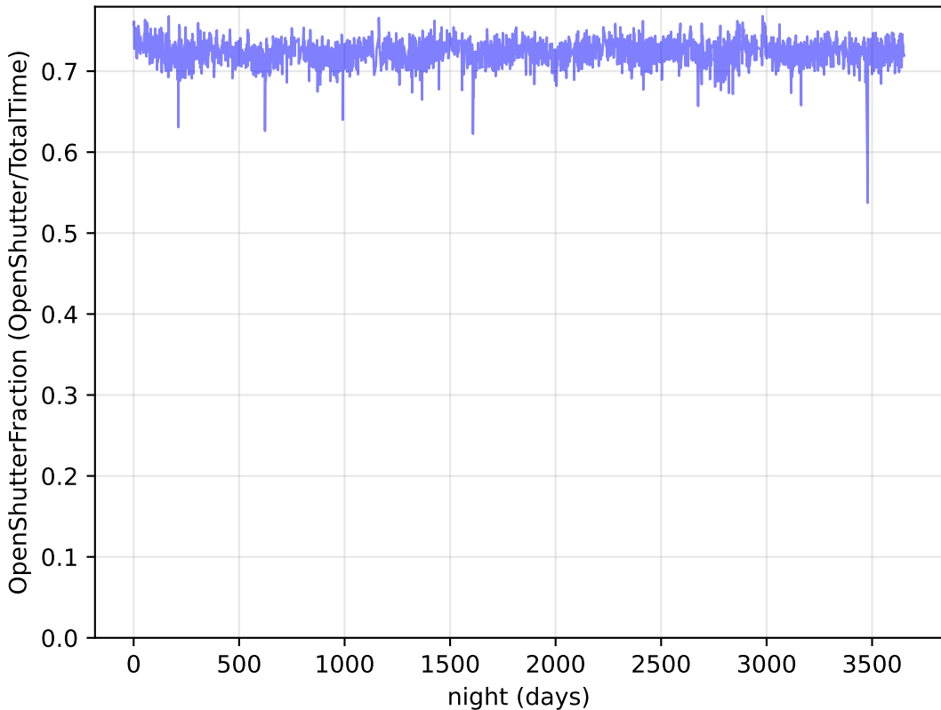
too_elab_r8_d3_ugrizy_v3.4_10yrs : OpenShutterFraction
