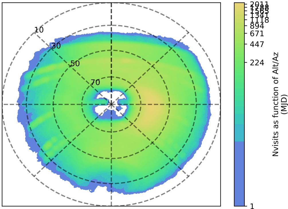
too_elab_r8_d3_ugrizy_v3.4_10yrs y: Nvisits as function of Alt/Az
