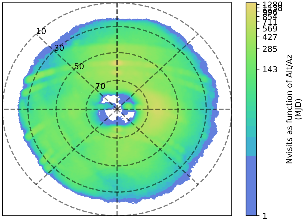
too_elab_r8_d3_ugrizy_v3.4_10yrs g: Nvisits as function of Alt/Az
