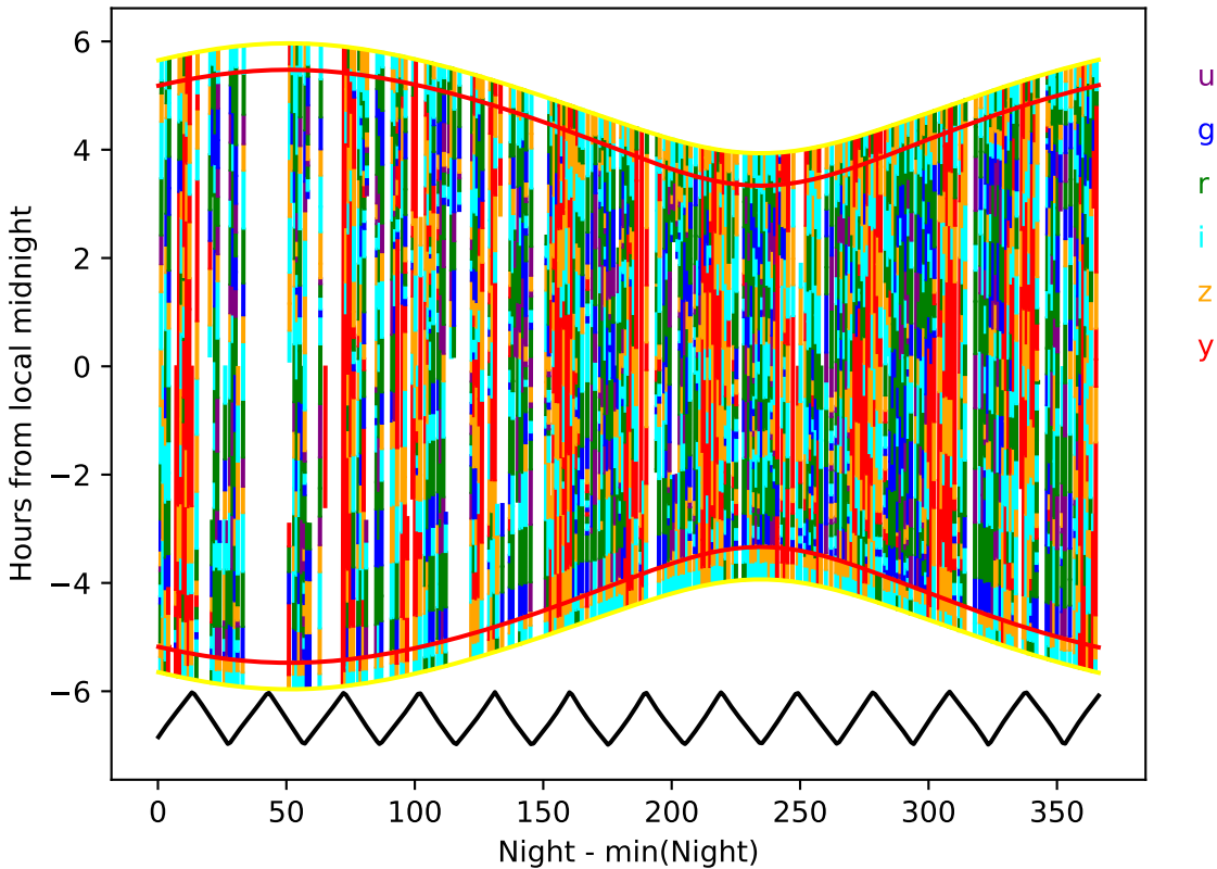
too_elab_r8_d3_ugrizy_v3.4_10yrs year 8-9: Hourglass
